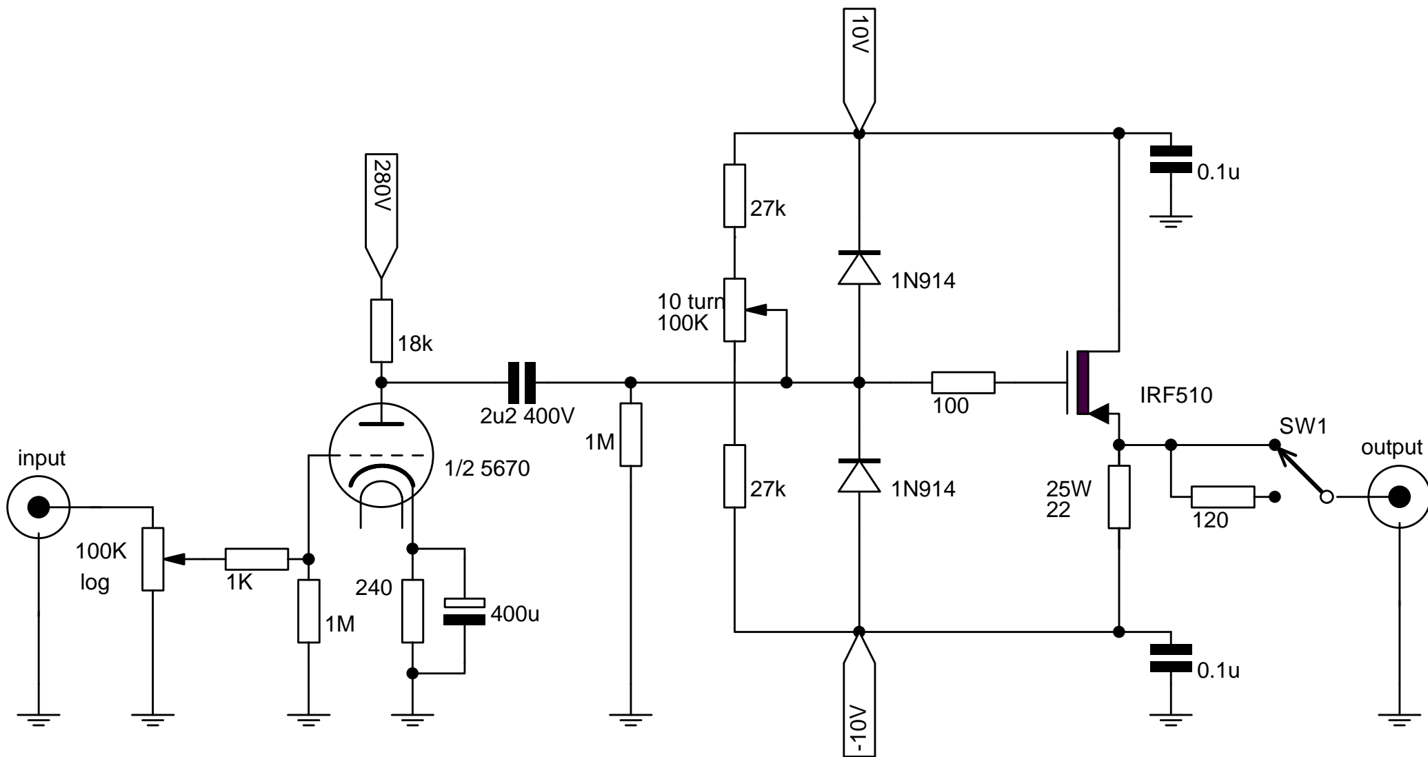
Hybrid 5670/Szekeres headphone amplifier (one channel)
